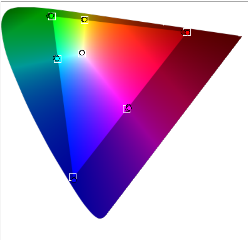
CIE 1976 u'v'
